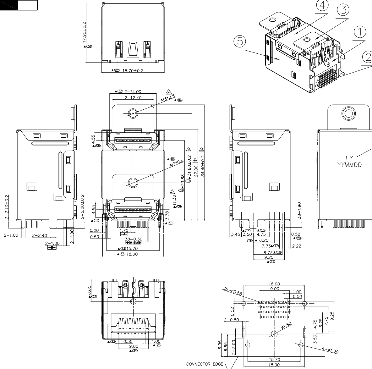
RECOMMENDED P.C.B LAYOUT T=1.60mm TOP VIEW (TOLRANCE:±0.05)
